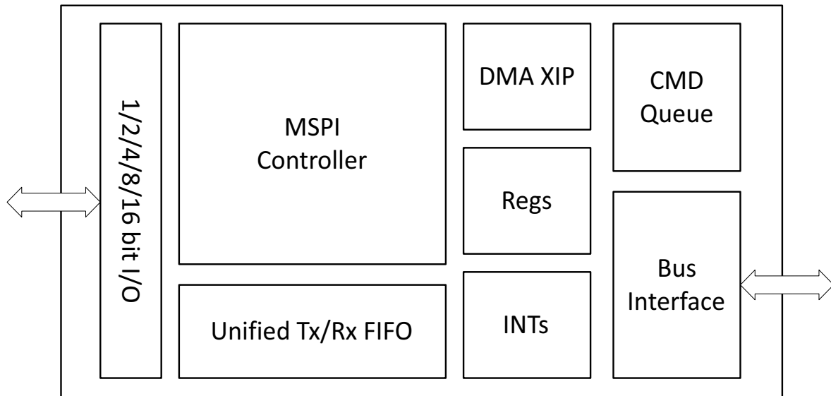
Figure 20. MSPI Module Block Diagram
