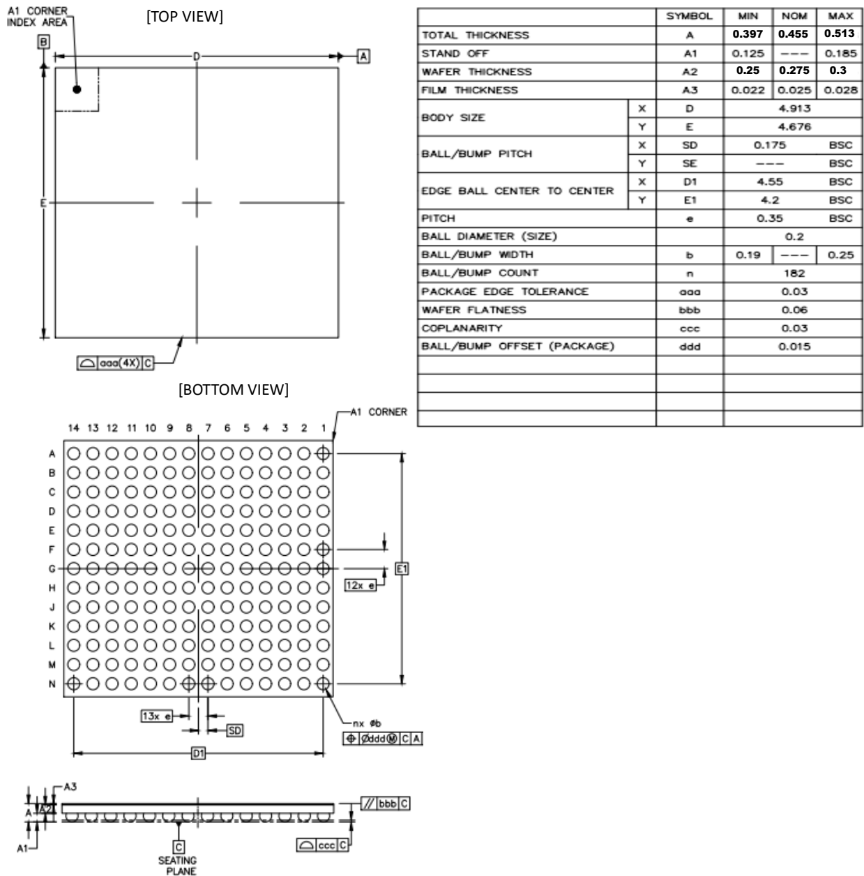
Figure 61. Apollo510 WLCSP Package Drawing
