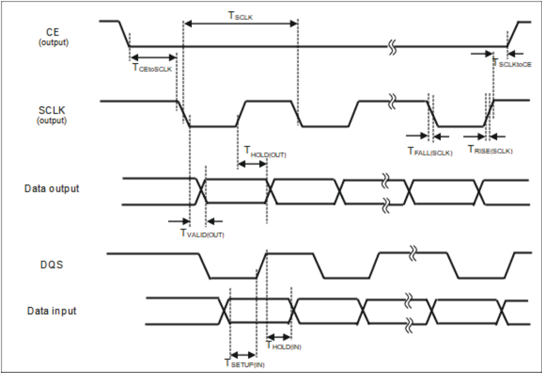
Figure 74. MSP11/MSP12 DDR with DQS Mode Timing Diagram
