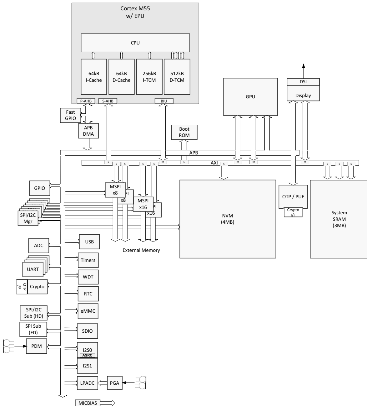
Figure 2. Apollo510 SoC Detailed Block Diagram
