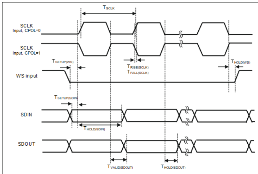
Figure 84. I 2 S Subordinate Interface Timing Diagram
