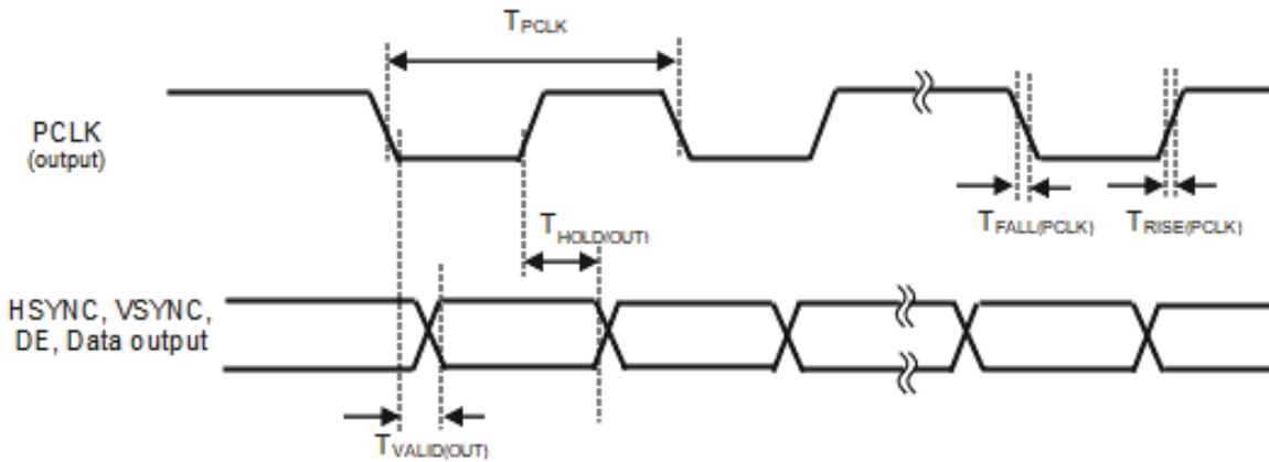
Figure 67. DC MIPI DPI-2 Timing Diagram
