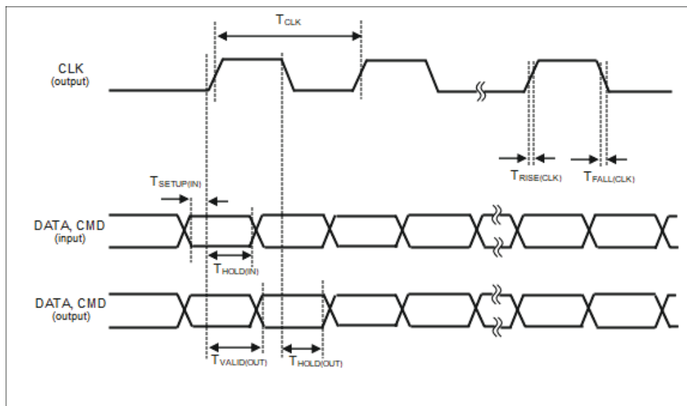
Figure 83. SD DDR50 Mode Interface Timing Diagram
