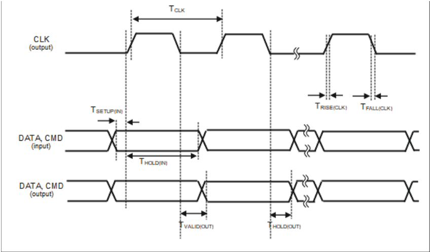
Figure 81. Default and High-Speed SD Interface Timing Diagram
