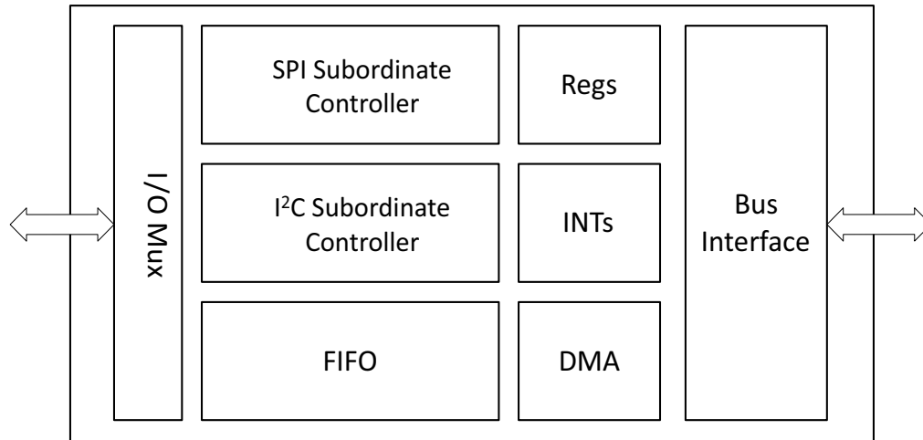
Figure 31. Block Diagram for IOS
