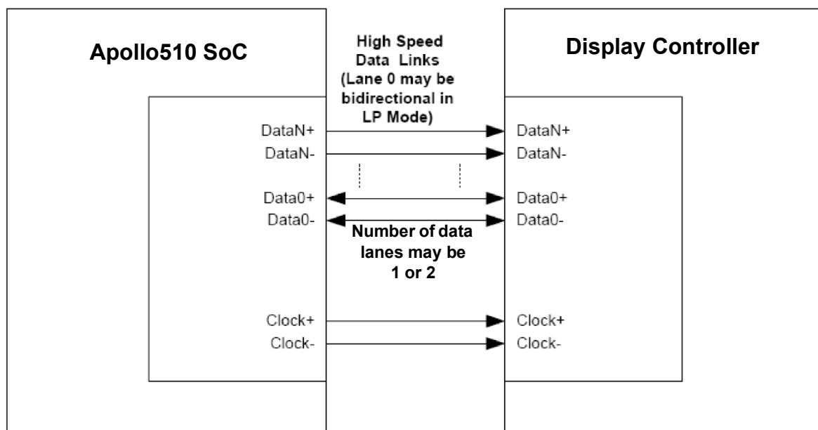
Figure 49. Display Serial Interface Bus with DSI Devices
