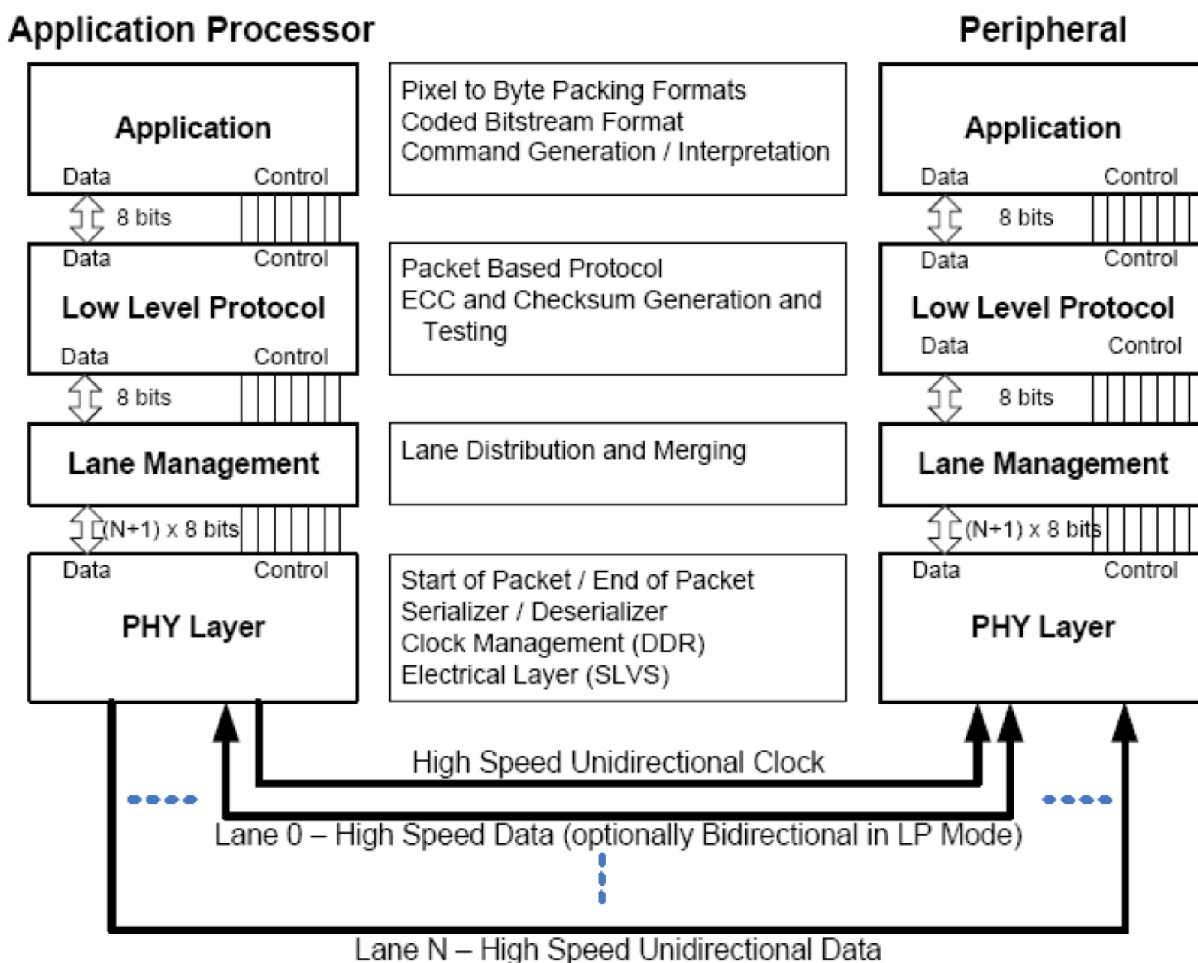
Figure 50. Layers in the DSI Data Transfer Model
