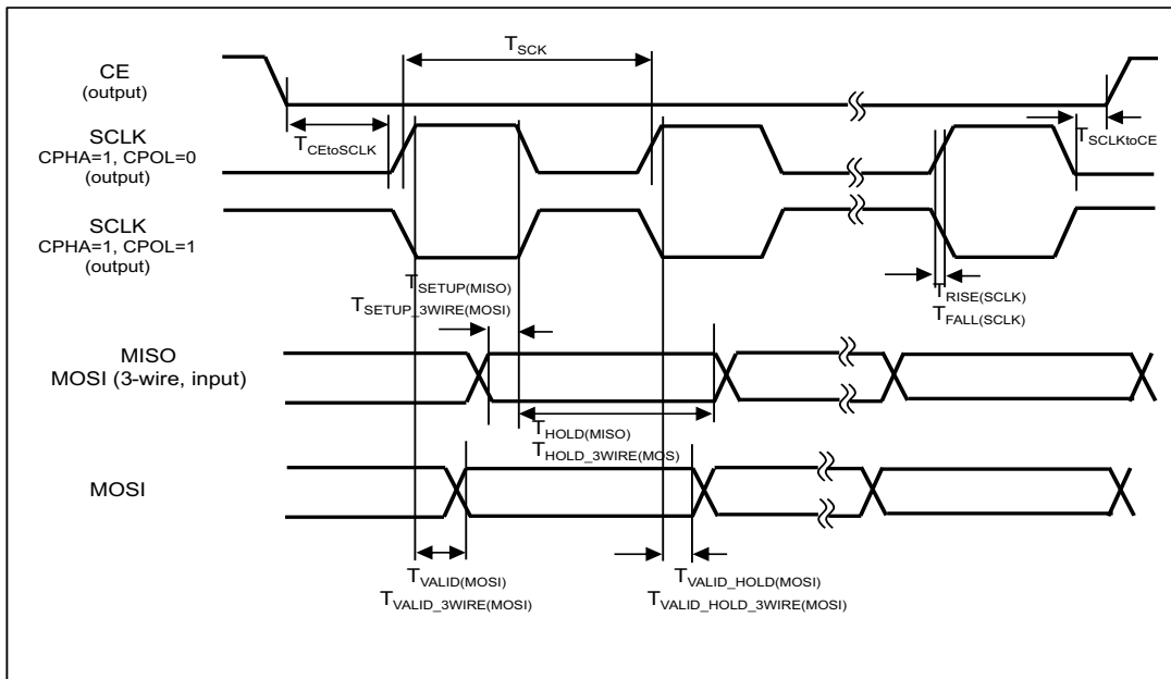
Figure 77. SPI Manager Interface Timing Diagram, CPHA = 1
