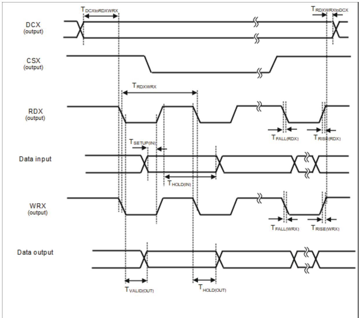
Figure 68. DC MIPI DBI-B Timing Diagram
