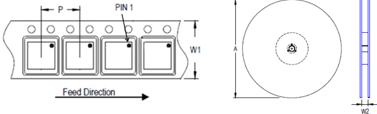
Figure 63. Tape Feed Direction and Reel Dimension Drawing
