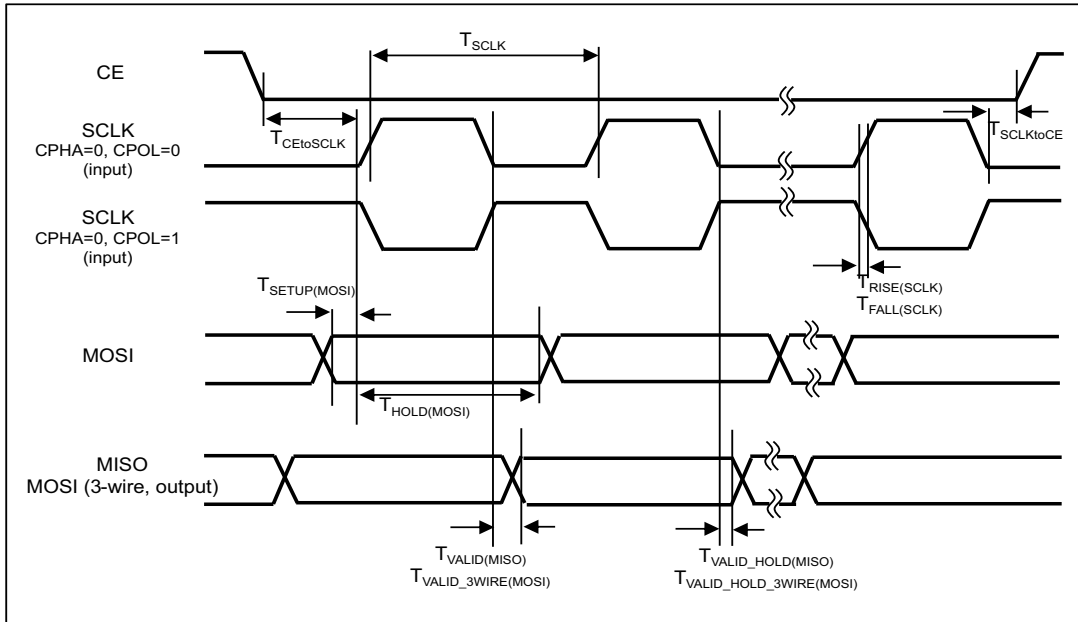
Figure 79. SPI Subordinate Interface Timing Diagram, CPHA = 0
