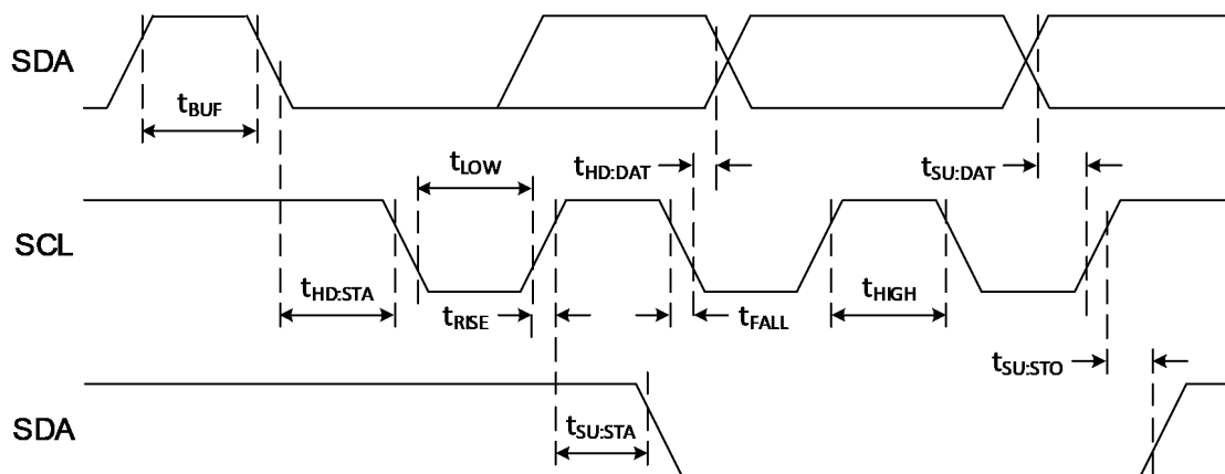
Figure 78. I 2 C Interface Timing Diagram
