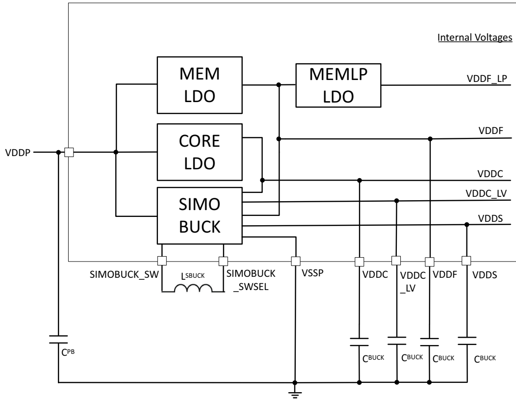
Figure 65. External Components for SIMO Buck
