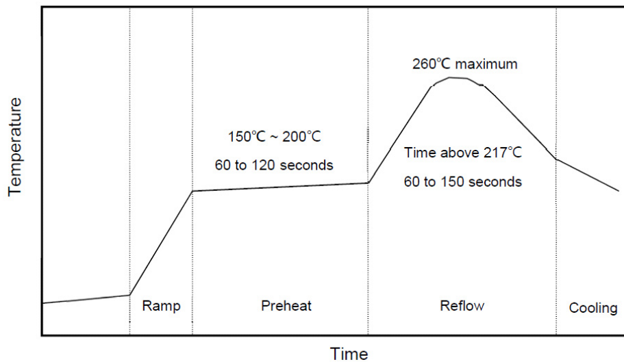
Figure 64. Reflow Profile
