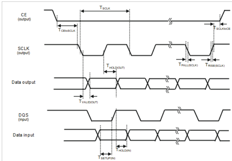
Figure 73. MSPI0/MSPI3 DDR with DQS Mode Timing Diagram
