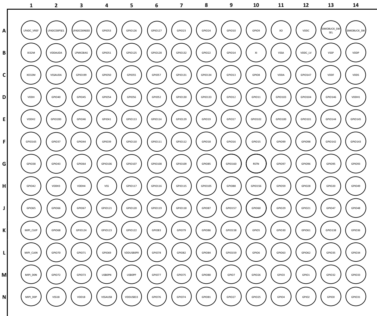
Figure 57. Apollo510 SoC WLCSP Pin Configuration Diagram - Top View
