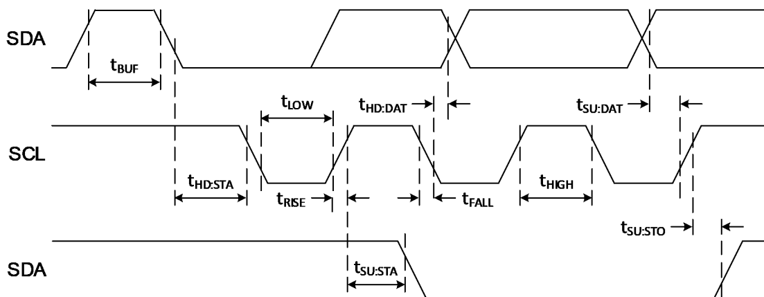
Figure 75. I 2 C Interface Timing Diagram
