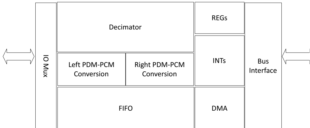
Figure 52. PDM Block Diagram
