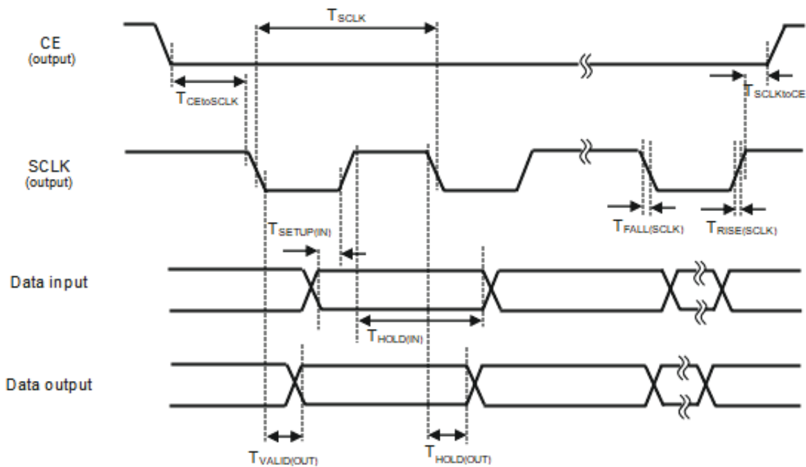
Figure 72. SDR Non-DQS Mode Timing Diagram (All MSPIs)
