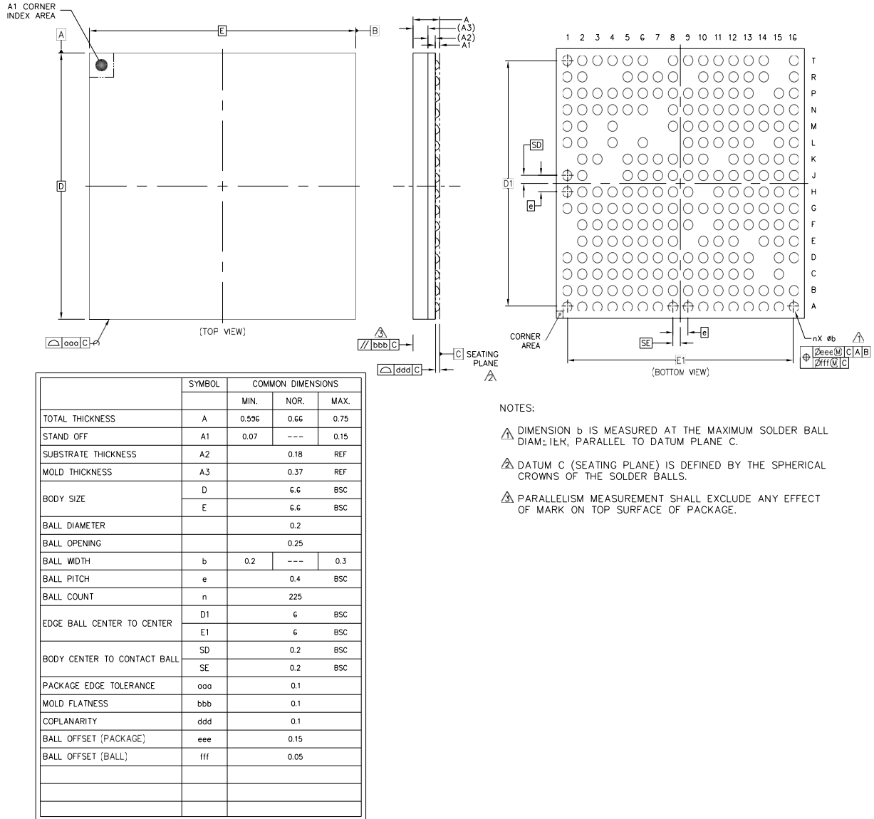
Figure 58. Apollo510 BGA Package Drawing
