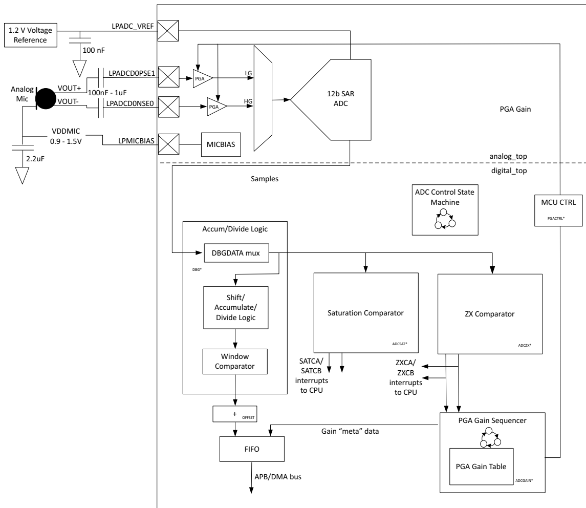
Figure 53. Low Power Analog Audio Interface Block Diagram
