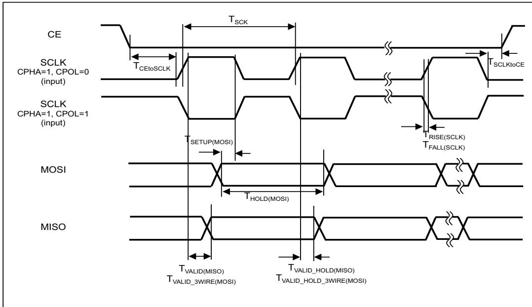
Figure 80. SPI Subordinate Interface Timing Diagram, CPHA = 1
