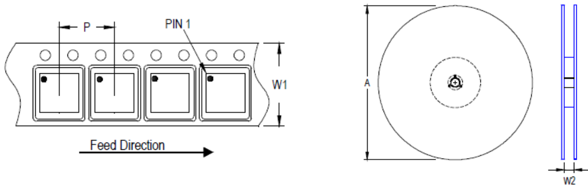
Figure 60. Tape Feed Direction and Reel Dimension Drawing
