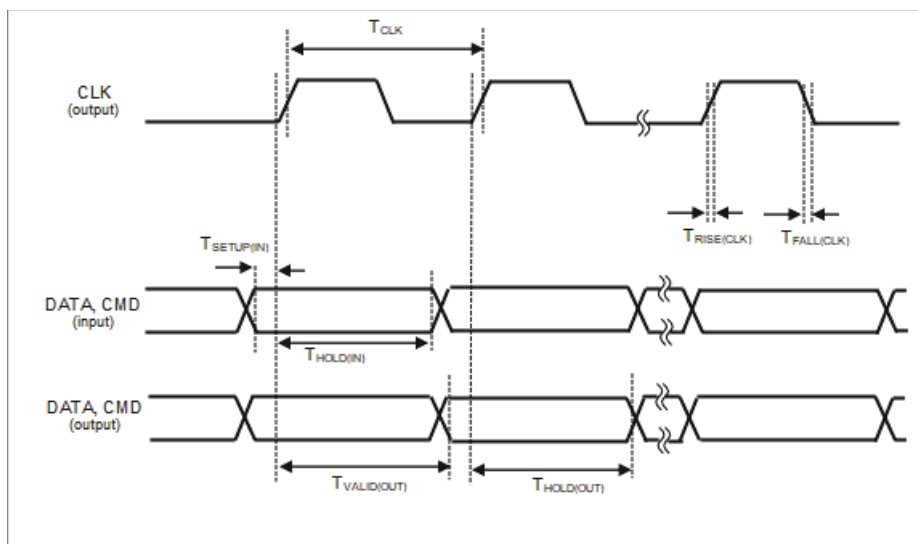
Figure 82. SD SDR50 Mode Interface Timing Diagram
