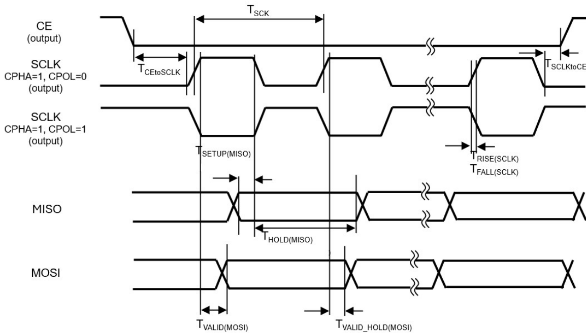
Figure 71. Standard 4-Wire Mode Timing Diagram, CPHA=1 (All MSPIs)
