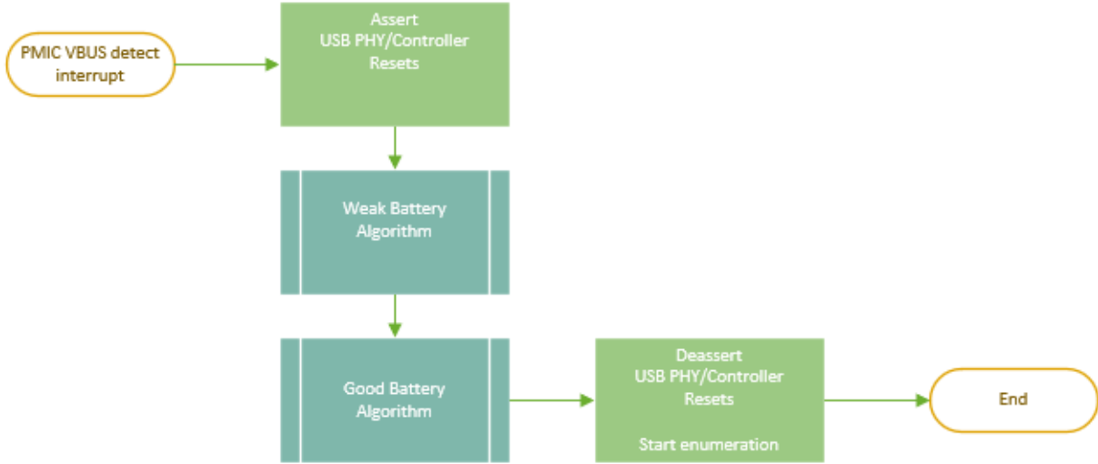
Figure 41. Charging Detection Algorithm
