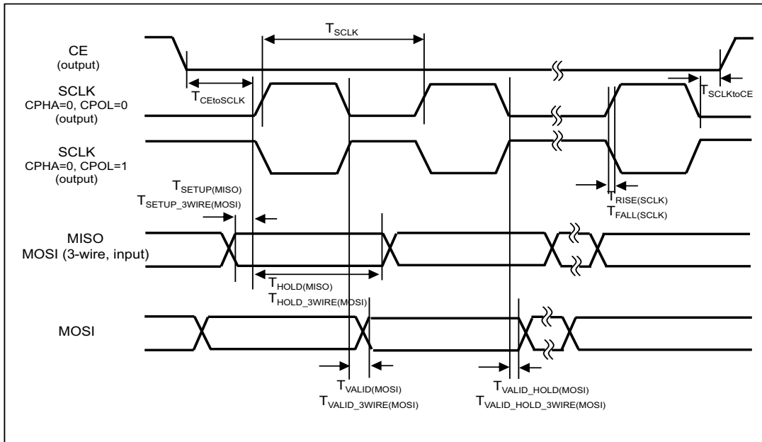
Figure 76. SPI Manager Interface Timing Diagram, CPHA = 0
