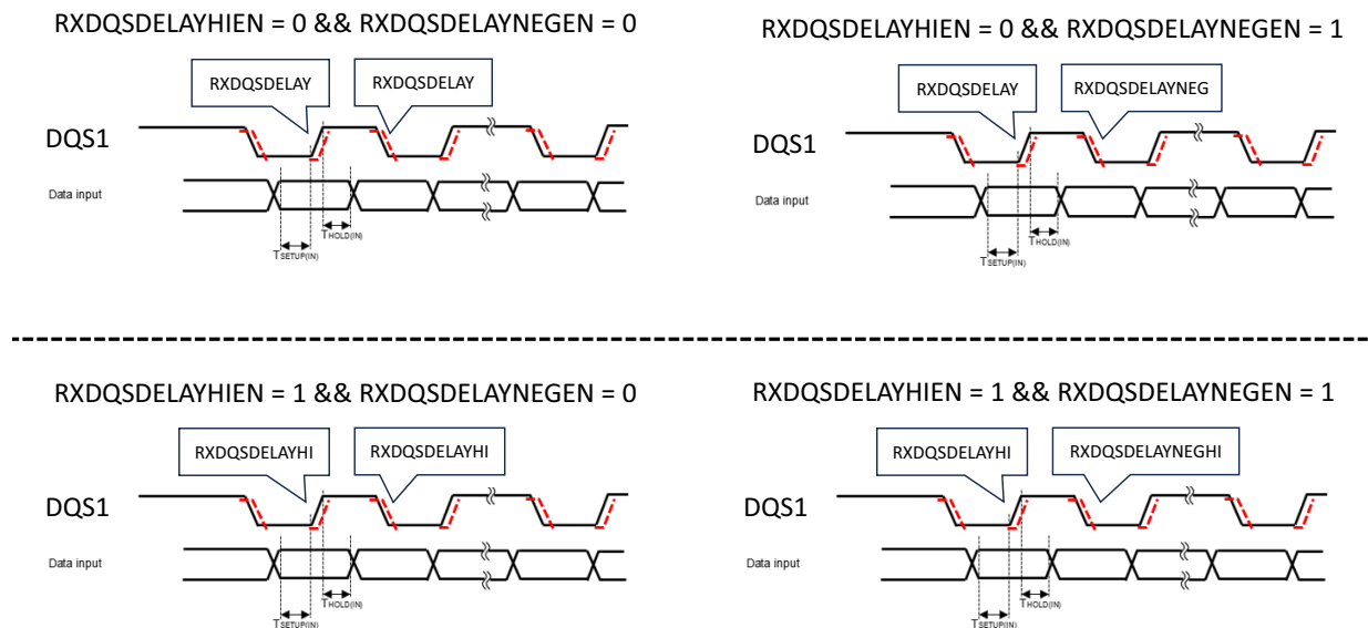
Figure 24. Hex DDR Mode with DQS - Read Delay Lines - Upper Data Byte DQS
