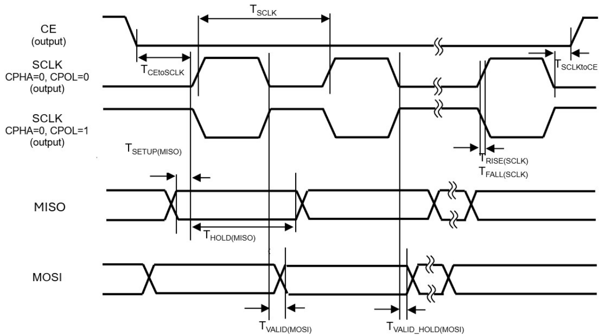
Figure 70. Standard 4-Wire Mode Timing Diagram, CPHA=0 (All MSPIs)
