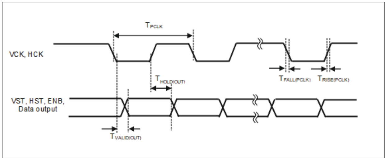
Figure 69. DC JDI MIP Timing Diagram
