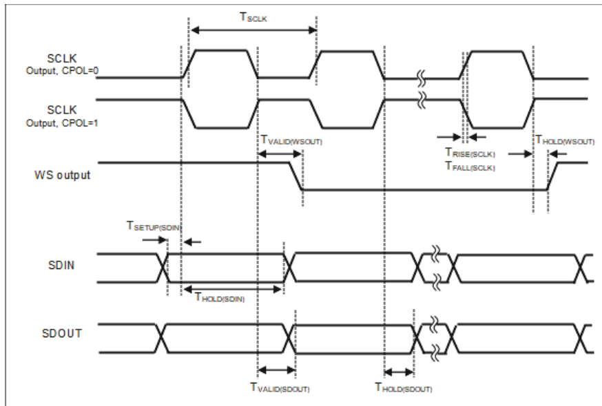
Figure 85. I 2 S Manager Interface Timing Diagram
