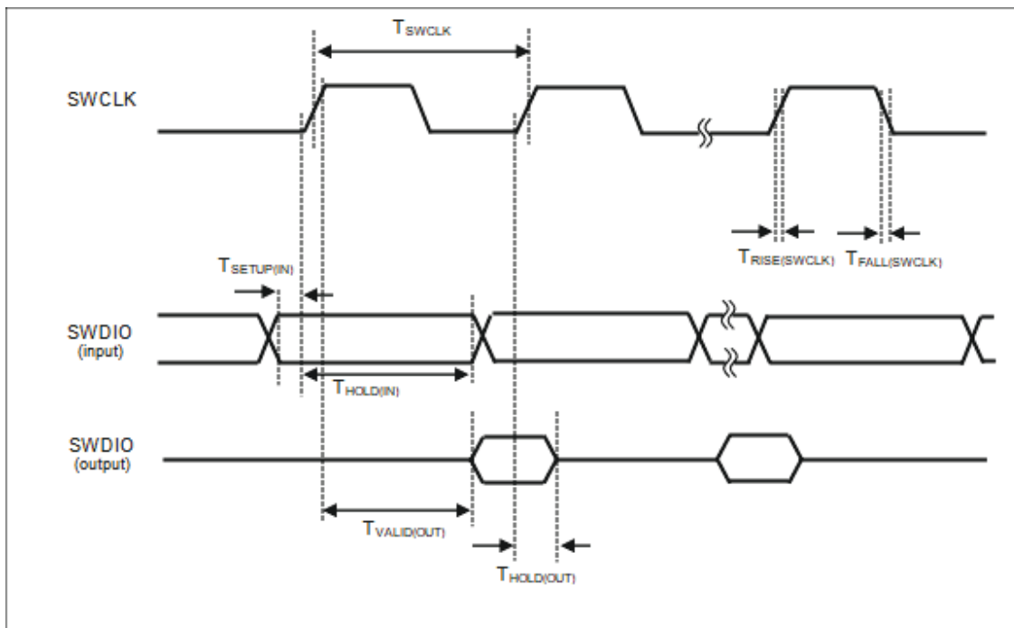
Figure 87. SWD Interface Timing Diagram
