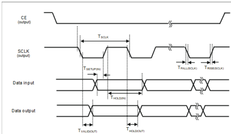
Figure 66. DC QSPI/SPI Timing Diagram
