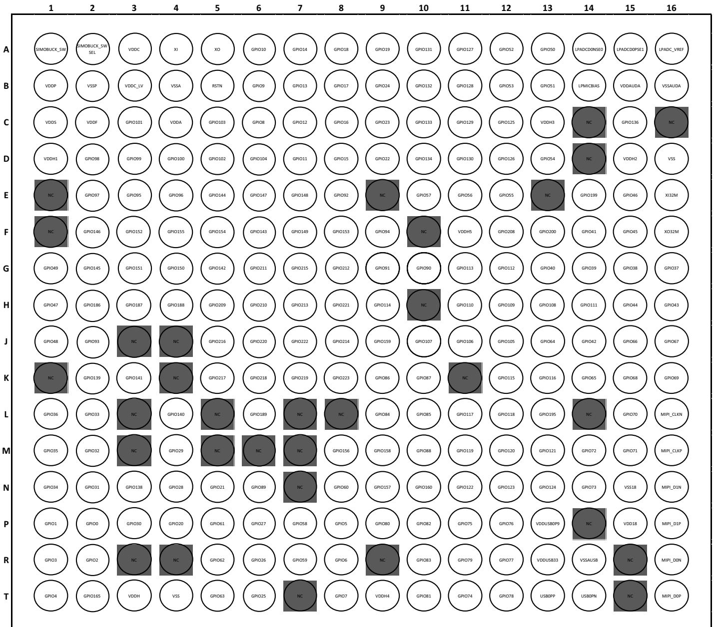
Figure 56. Apollo510 SoC BGA Pin Configuration Diagram - Top View
