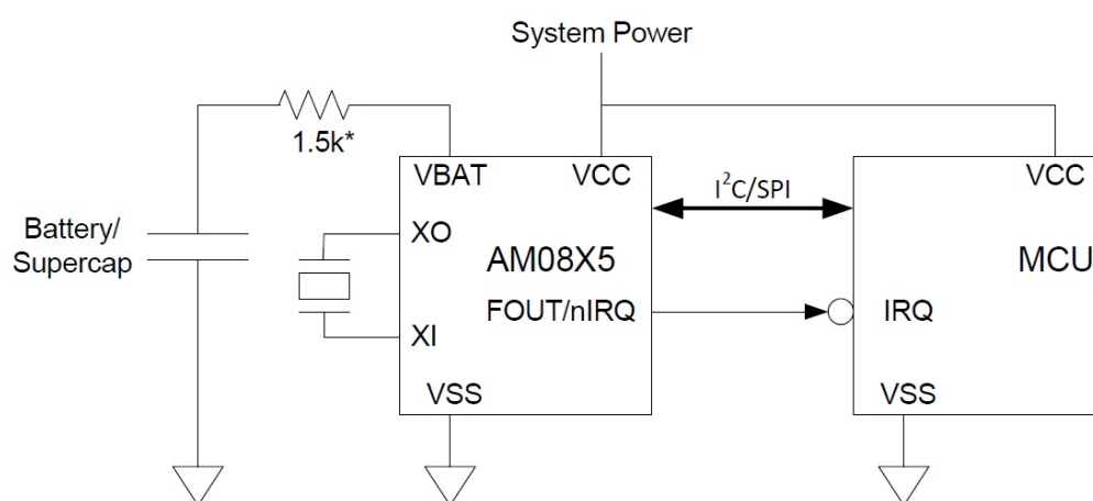
Figure 1-1: Typical Application Circuits
