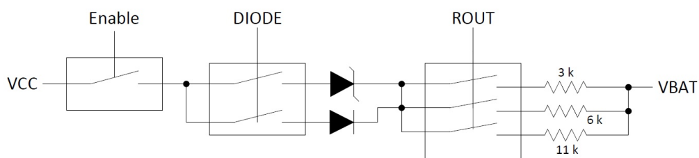
Figure 5-12: Trickle Charger
