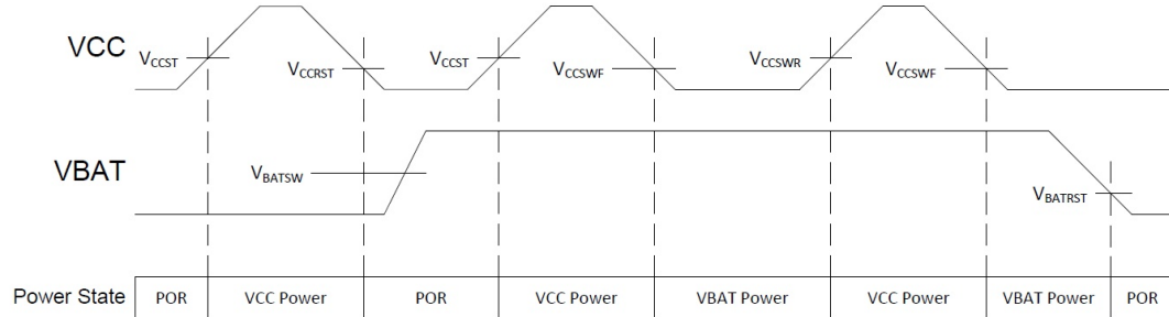
Figure 4-1: Power Supply Switchover
