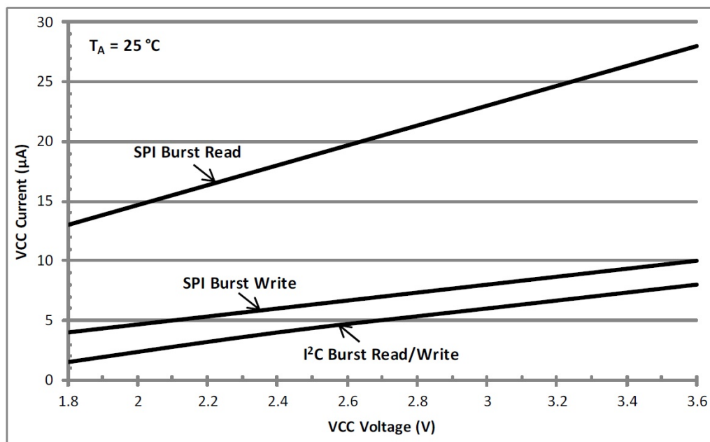
Figure 4-8: Typical VCC Current vs. Voltage, I 2 C and SPI Burst Read/Write
