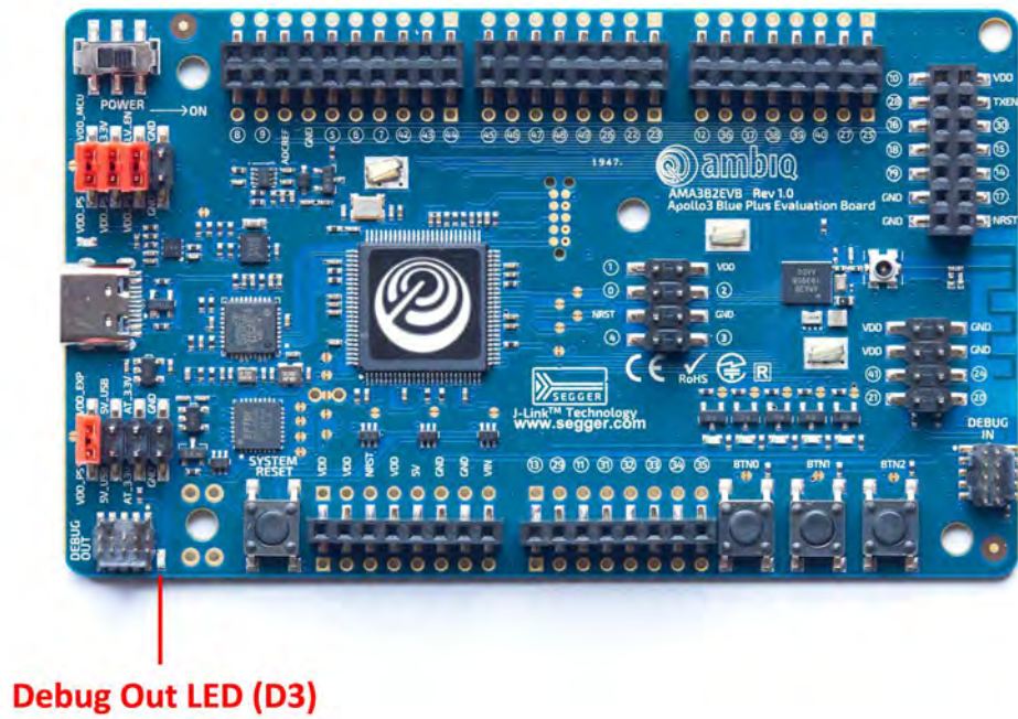
Figure 3-3: Apollo3 Blue Plus EVB's DEBUG OUT LED (D3)
