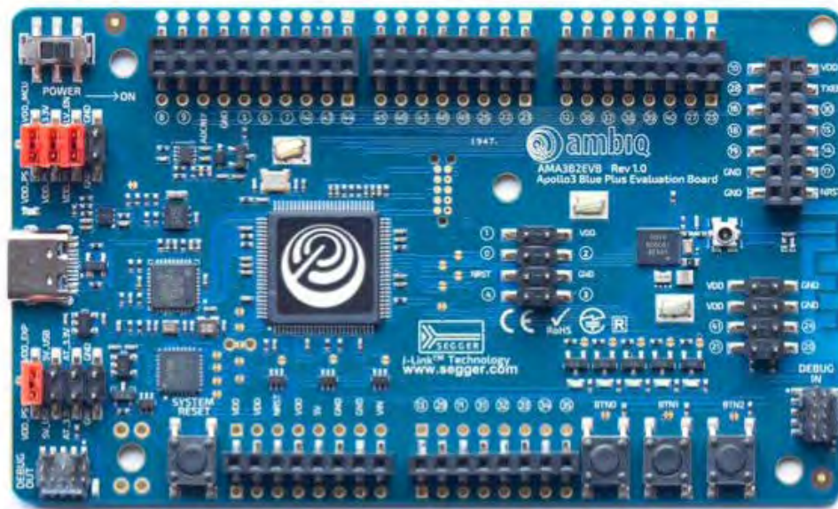
Figure 2-1: Apollo3 Blue Plus EVB, Revision 1.0
