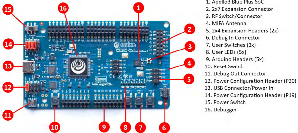
Figure 2-2: Apollo3 Blue Plus EVB Parts Diagram
