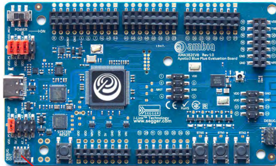
Figure 3-2: Apollo3 Blue Plus EVB's DEBUG OUT Header (J2)
