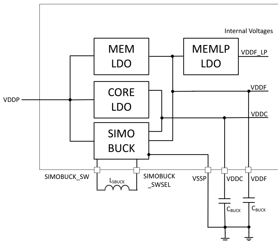
Figure 58. External Components for SIMO Buck
