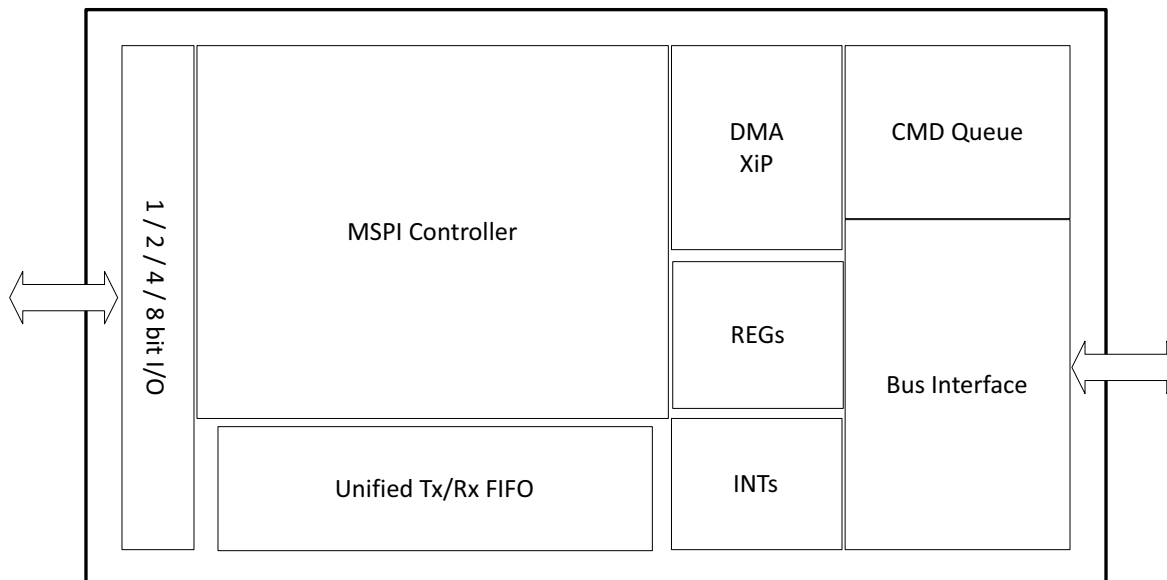
Figure 22. Block Diagram for the MSPI Master Module
