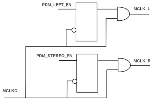
Figure 50. PDM Converter Core Local Clock Gating
